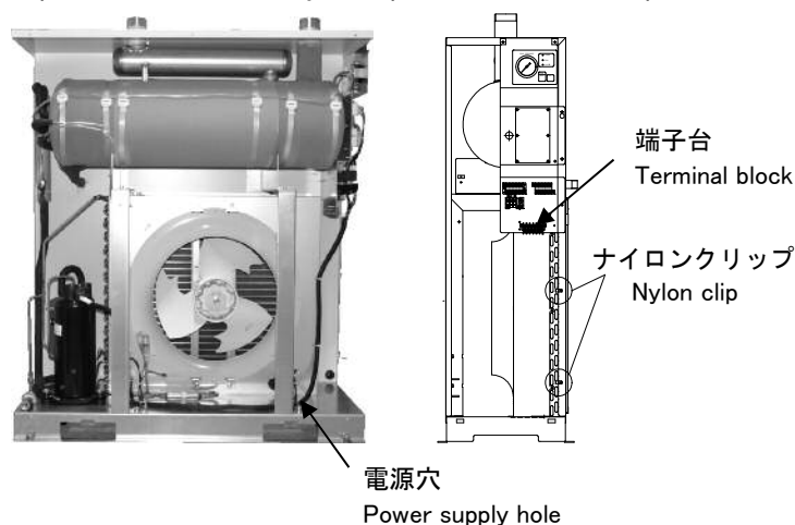
端子台仕様 Specification of the terminal block.
