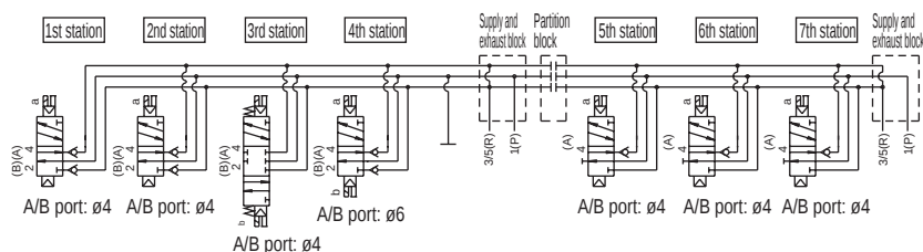
Reference circuit diagram Simplified circuit diagram of manifold model No. (example) from previous page
