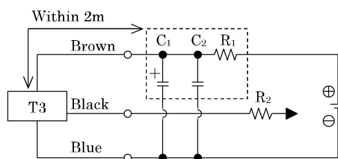
Fig. 10 • Electric power noise absorptive circuit. C_1 =20 to 50 \mu F electrolytic capacitor (Withstand voltage 50V or more) C_2 =0.01 to 0.1 \mu F ceramic capacitor R_1 =20 to 30 \Omega • Dash current restriction resistor. R_2 =As much large resistor as the load circuit can afford. • Install it nearby the switch (Within 2m)
