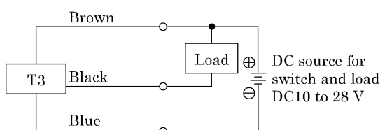
Fig. 3 T3 Fundamental circuit Example (1) (In case the same source of power is used.)
