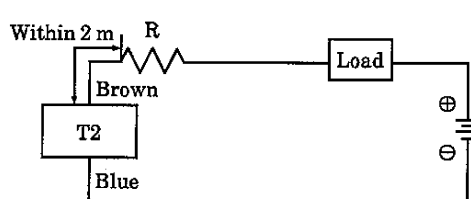
Fig.6 • Dash current restriction resistor R = As much large resistor as the load circuit can afford. • Install it nearby the switch (within 2 m).
