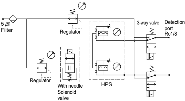
Fig. 2 Circuit for detection and air blow
