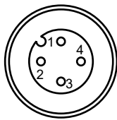
Fig. 3 Connector pin array (body side)
