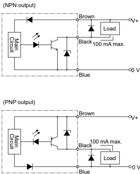
Fig. 6 Output circuit
