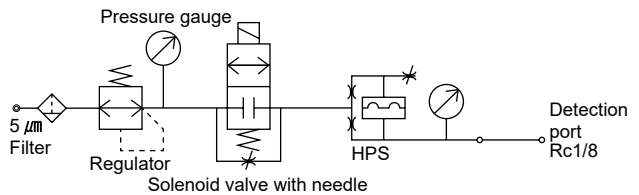
Fig. 1 Recommended circuit
