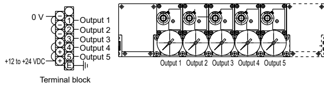
Fig. 5 Terminal box layout
