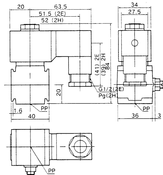
Figure 30 GPS2-AB3X-2E(2H)-DC24V
