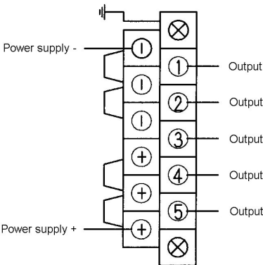
Terminal arrangement
