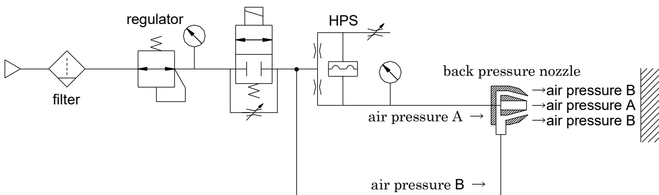
Figure 1 Standard circuit with back pressure nozzle
