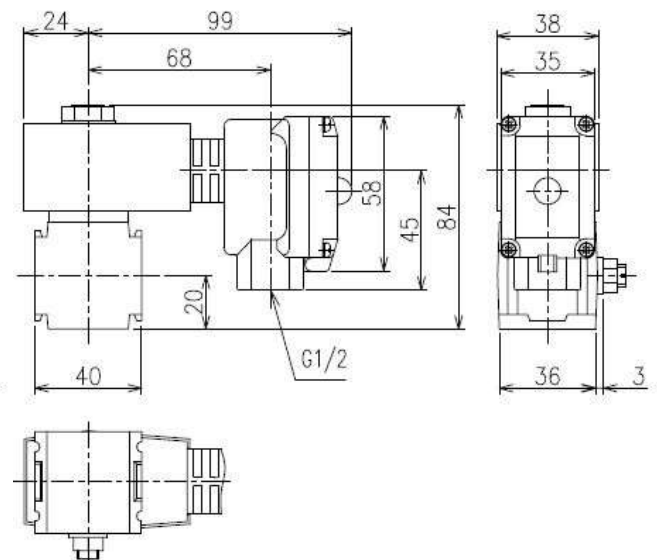
Figure 32 GPS2-AB3X-3N-DC24V
