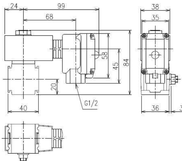
Figure 31 GPS2-AB3X-3N-AC100V(AC200V)
