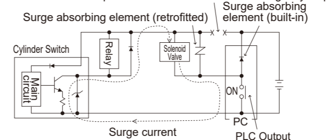
Circuit interruption due to disconnection or emergency stop
