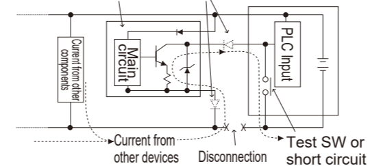
Cylinder switch Reverse current prevention diode Control panel
