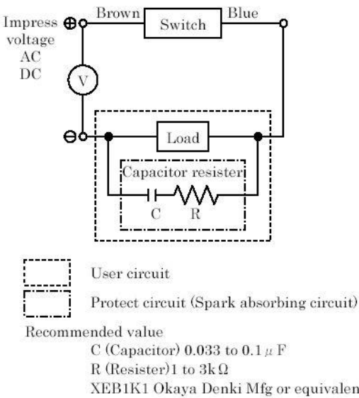
Fig.1 When capacitor resistor is used.
