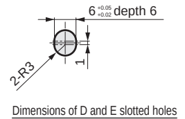
Dimensions of D and E slotted holes
