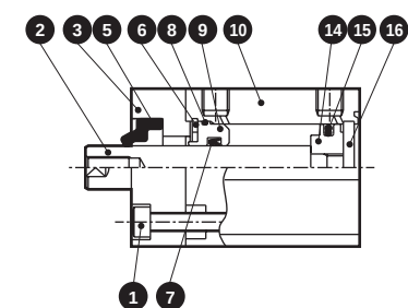
● SSD-G \frac{2}{3} -16 (without switch)
