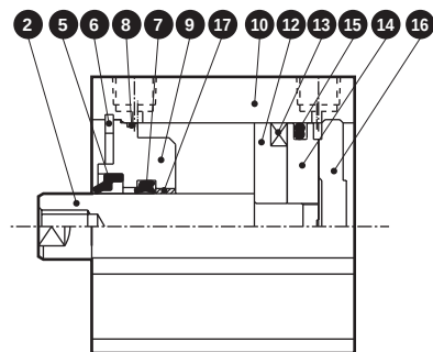
● SSD-G \frac{2}{3} L-63 to 100 (with switch)
