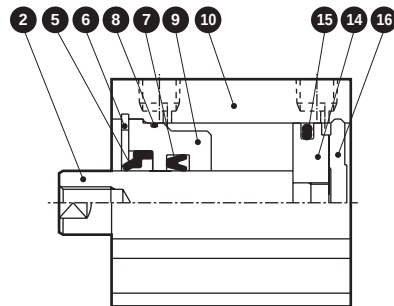
● SSD-G \frac{2}{3} -32 to 50 (without switch)
