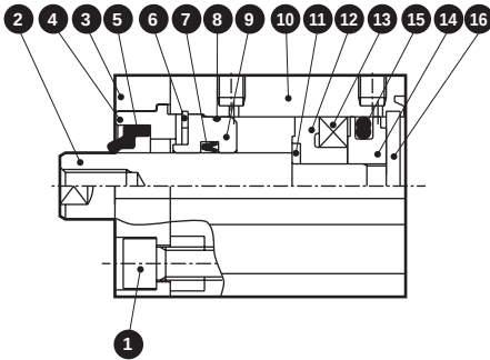
● SSD-G \frac{2}{3} L-20, 25 (with switch)
