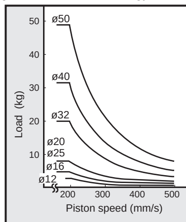
High load allowable energy value graph
