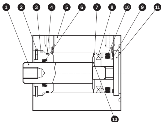
● SSD-OL-32 to 50 (double acting/low speed/with switch)
