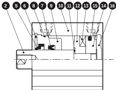
● SSD-G \frac{2}{3} L-32 to 50 (with switch)
