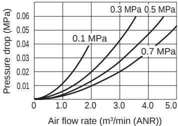
● FW4000-15-W
