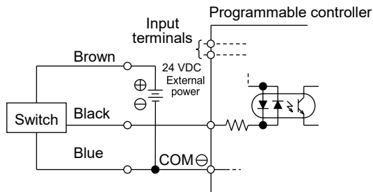
3-wire connection to source input (internal power)
