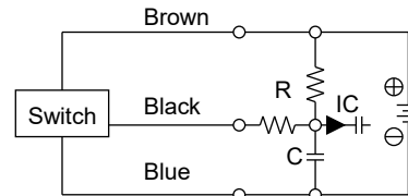
Ex. 2 Using capacious load with current regulating resistor R. Use the following formula to figure out resistance R ( \Omega ).
