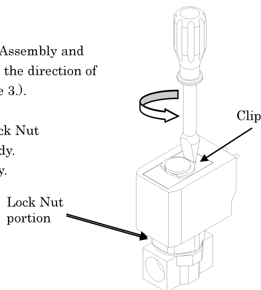
(Figure 3.) How to disassemble the Clip
