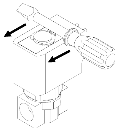
(Figure 4.) How to assemble the Clip
