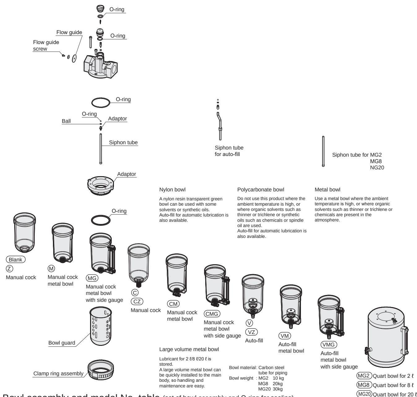
Bowl assembly and model No. table (set of bowl assembly and O-ring for sealing)
