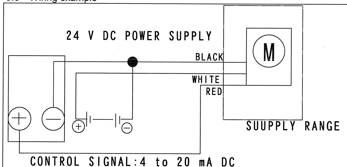
(FIG. 5.1 Wiring diagram)
