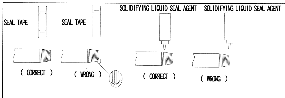
(FIG. 6.3 Sealing agent)
