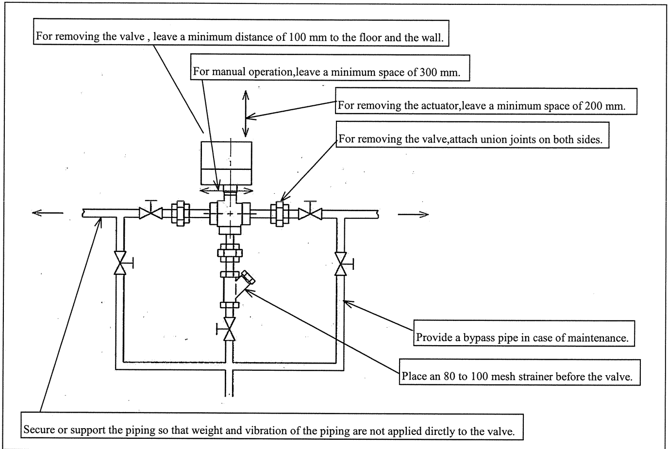
(FIG. 6.1 Piping example)
