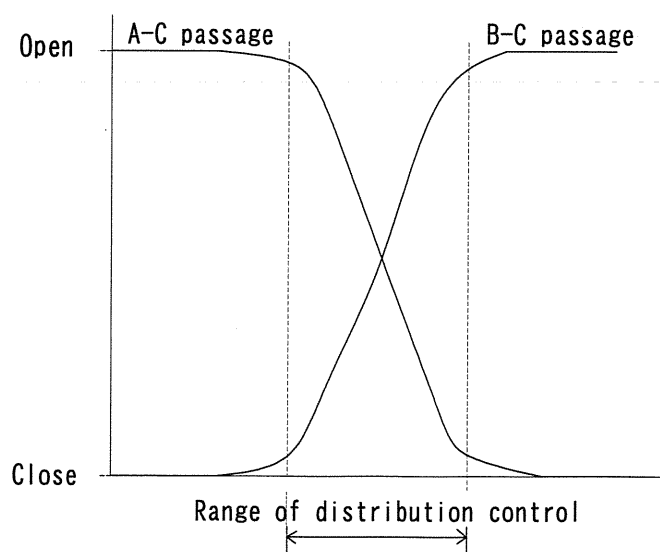
FIG. 11.2 Flow rate characteristic
