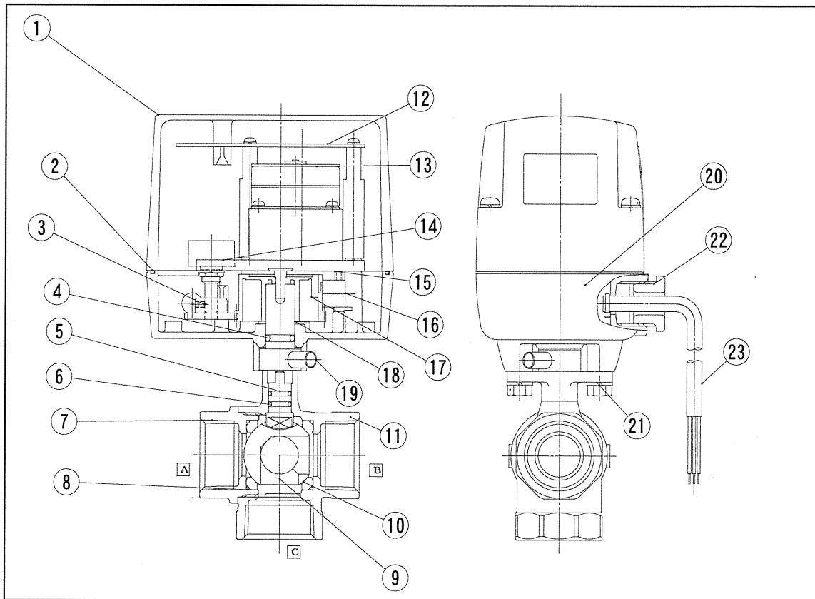
FIG. 13.1 Structural drawing
